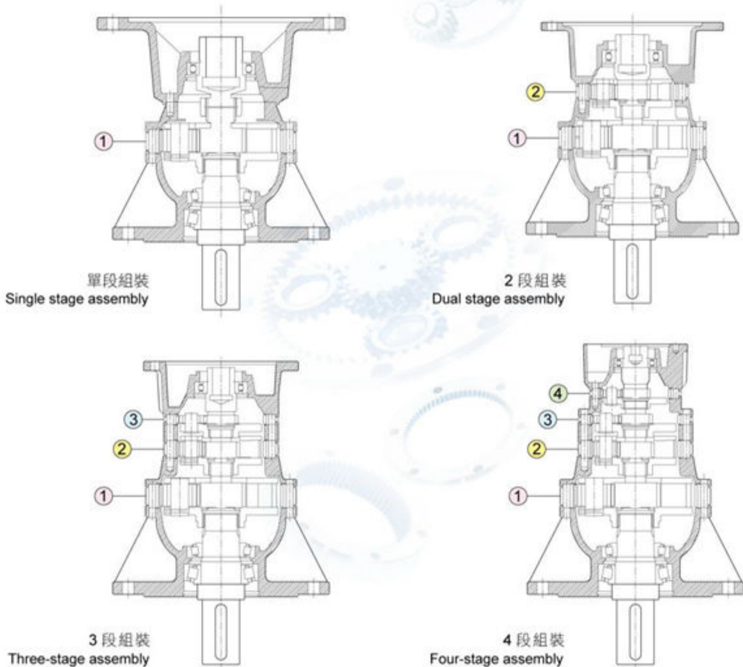
Staged assembly drawings of planetary speed reducers
