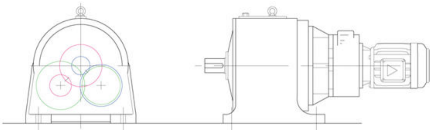
齒輪減速機 (Geared Speed Reducer)
